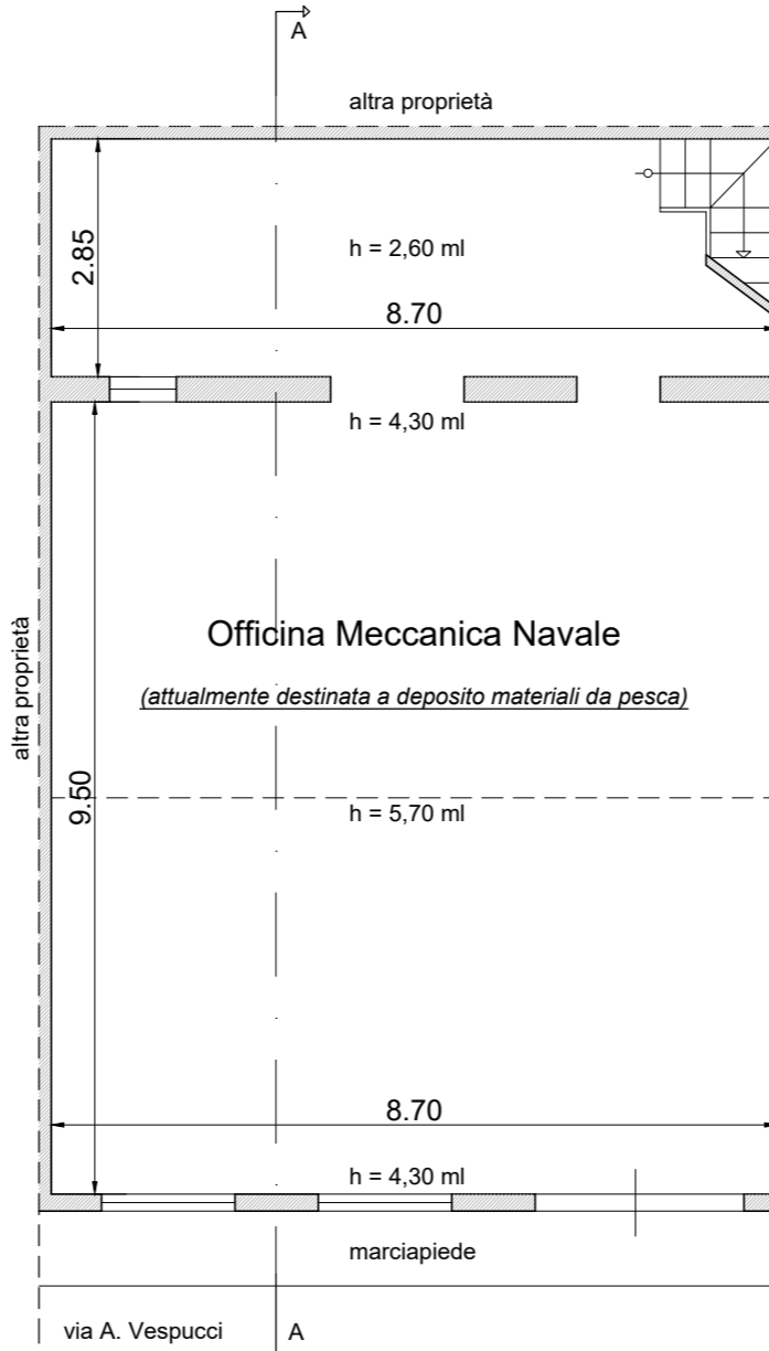
PIANO TERRA
