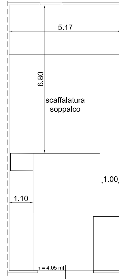
Pianta Piano Soppalco
