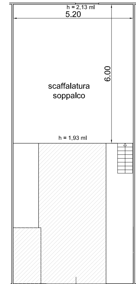
Pianta Piano Soppalco
